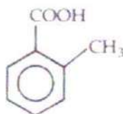
o-Toluic acid
