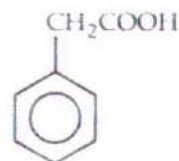
Phenyl acetic acid
