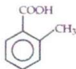
Methyl benzoic acid (Toluic acid)
