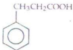
3-phenyl propanoic acid
